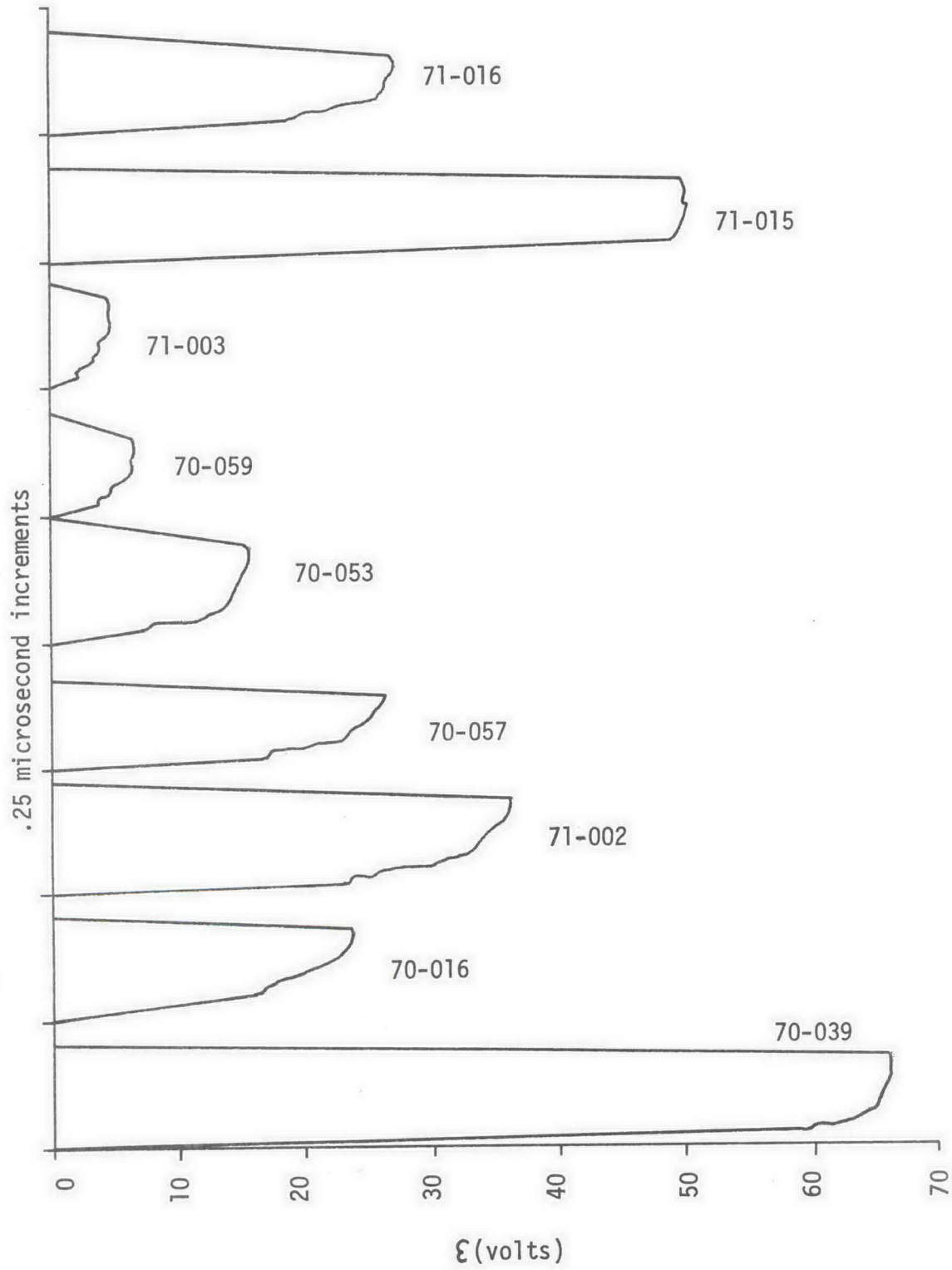
Fig. 5.5.--Oscilloscope profiles of the demagnetization process for the data presented in Table 4.
